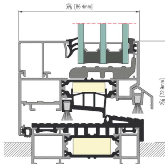
PERFORMANCE TM 77 BALCONY TILT&TURN WINDOW
