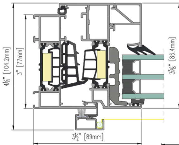
PERFORMANCE TM 77 TILT&TURN WINDOW WITH INSECT SCREEN
