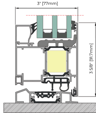
PERFORMANCE TM 77 DOOR (OUTWARD OPENING) WITH THRESHOLD
