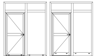
SINGLE DOOR WITH SIDELIGHT AND TRANSOM
