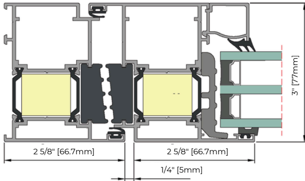
PERFORMANCE TM 77 DOOR (INWARD OPENING)
