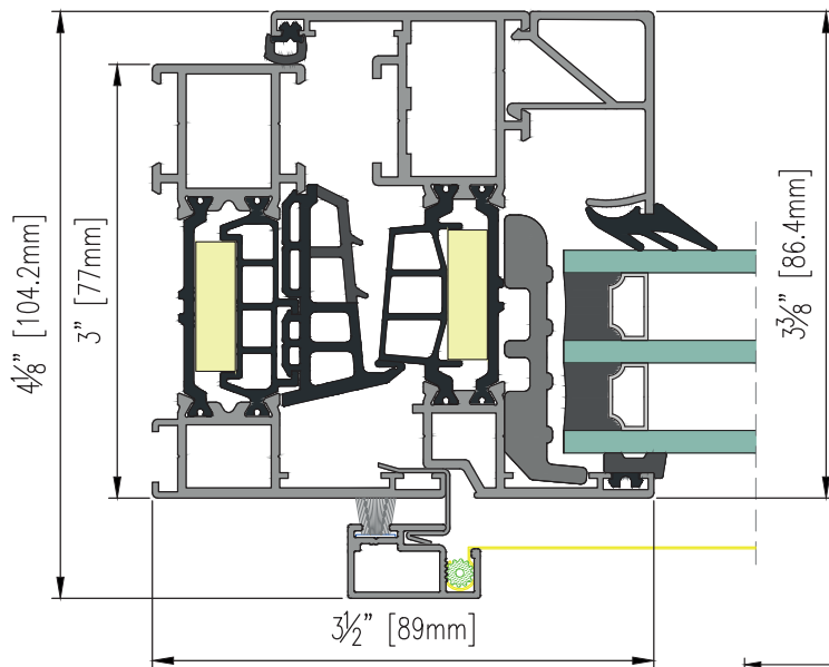
PERFORMANCE TILT&TURN WINDOW WITH INSECT SCREEN
