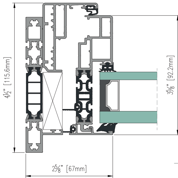
MOREVIEW CASEMENT WINDOW
