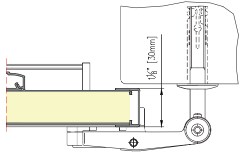
ECLIPSE FIXED LAMELLAR
