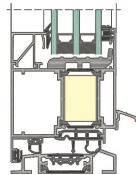
SECTION OF THE PANO GLASS DOOR
