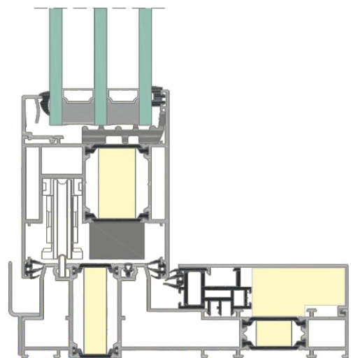
SECTION OF THE PANO LIFT'N'SLIDE DOOR
