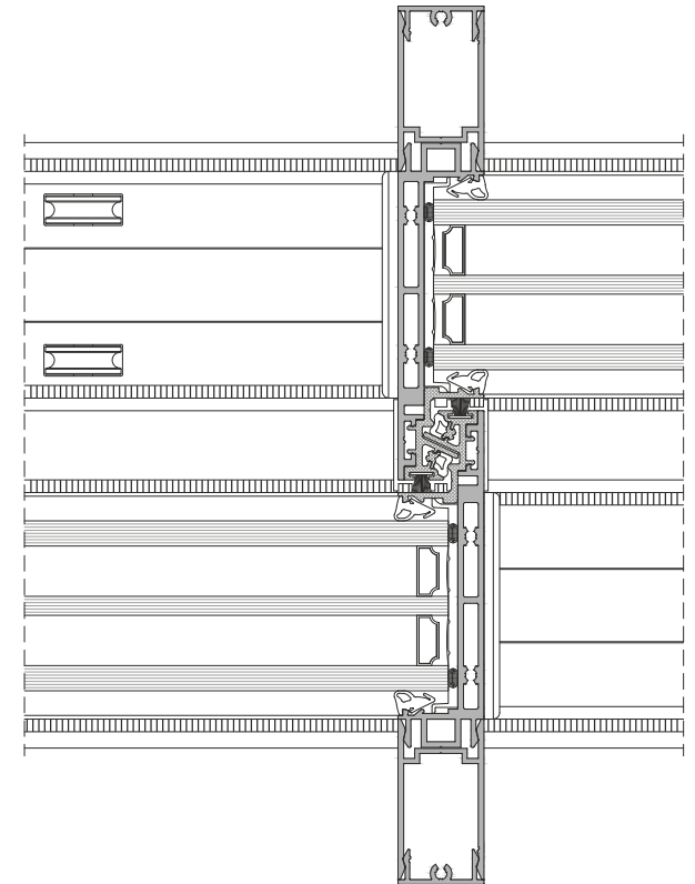
Cross-section through the leafs assembly
