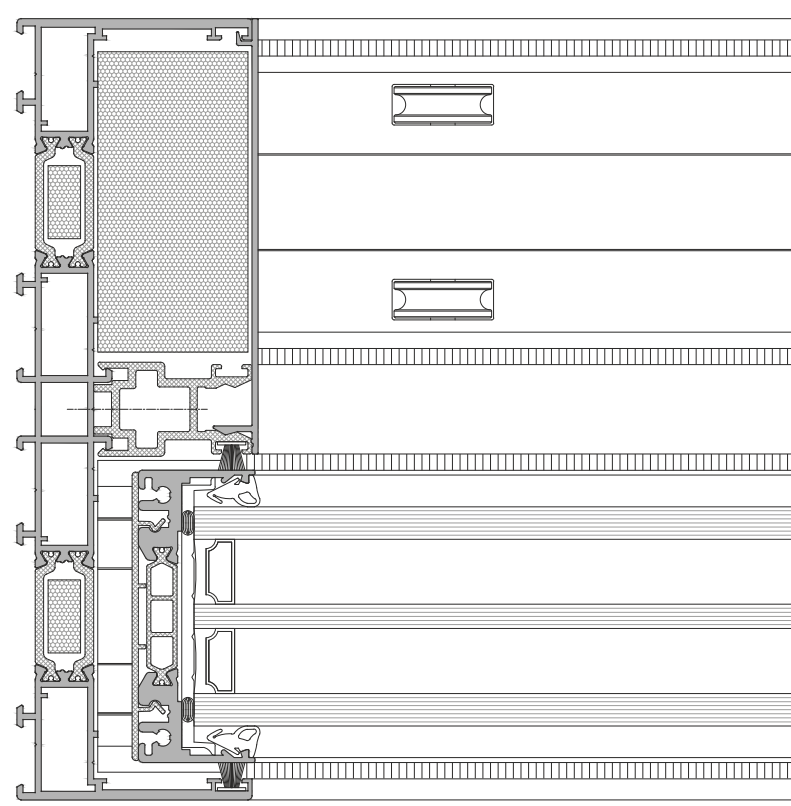
Lateral cross-section
