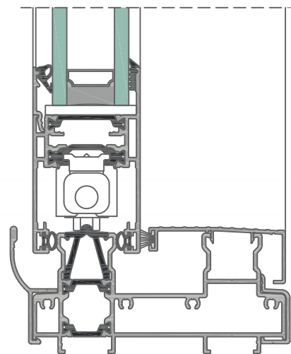
CROSS SECTION OF DOOR SCENIC SLIDER
