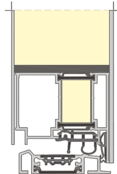
CROSS SECTION OF DOOR PRESTIGE - THRESHOLD SOLUTION
