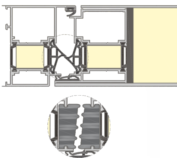
CROSS SECTION OF EXTERNAL DOOR PRESTIGE
